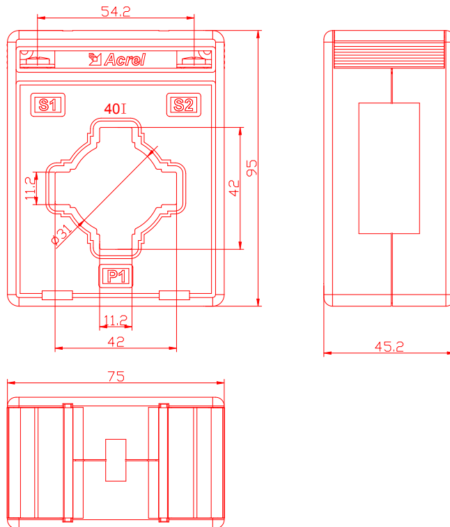
Figure 4 Outline dimensions of outlay current transformer
