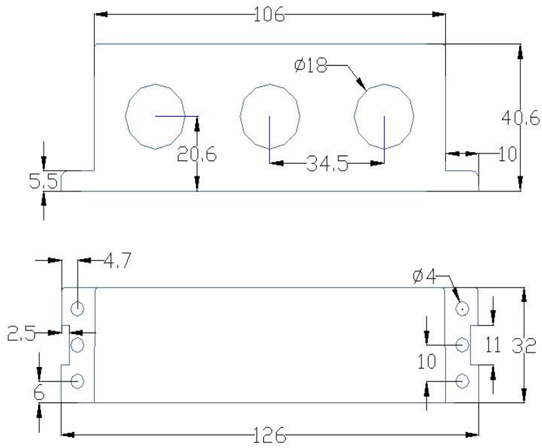
Figure 3 Transformer mounting dimension of less than 100A
