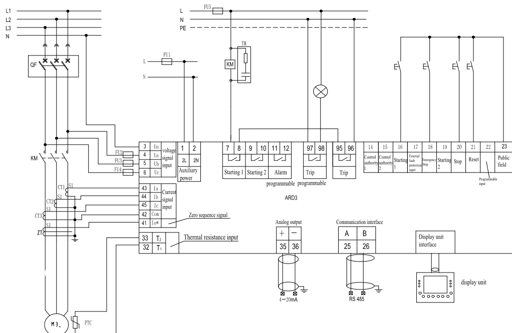
ARD3 motor protector direct starting mode wiring diagram
